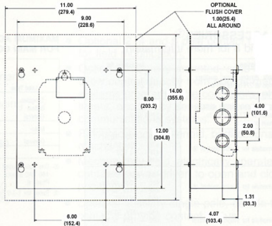
ASCO 917 ENCLOSED TYPE
