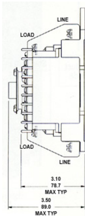
ASCO 917 OPEN TYPE SIDE VIEW
